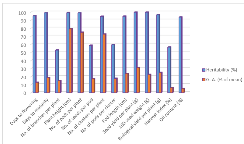
Fig 2: Graphical representation of heritability and genetic advance expressed as % of mean for various characters in soybean
